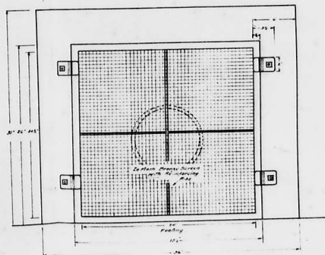
DETAIL OF INTAKE AND SCREEN
