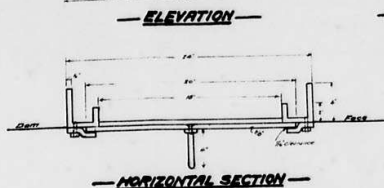
DETAIL OF SLUICWAY AND GATE
